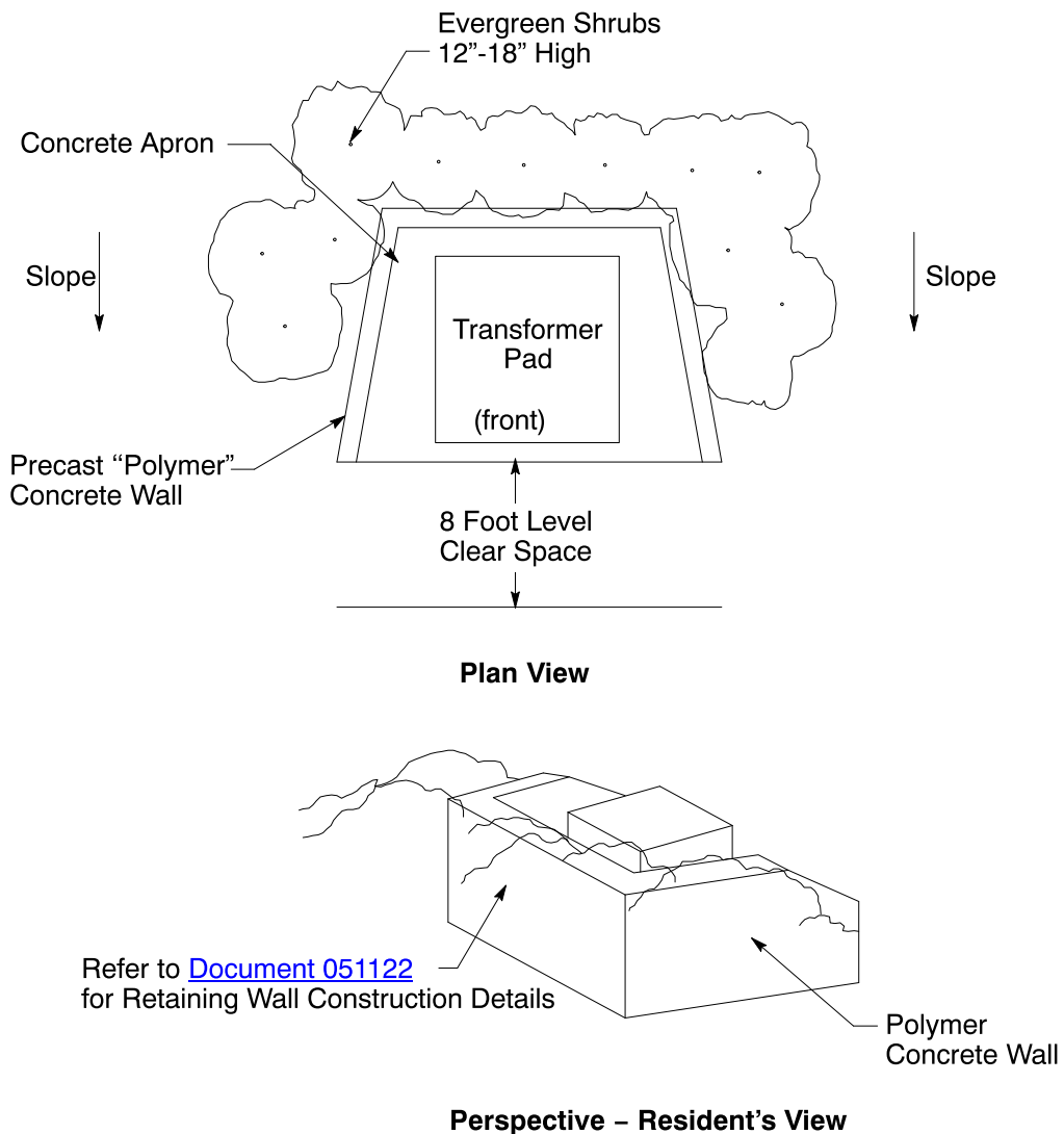
Figure 4 Retaining Wall
