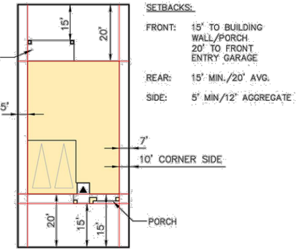
TYPICAL MINIMUM LOT SETBACKS N.T.S.
